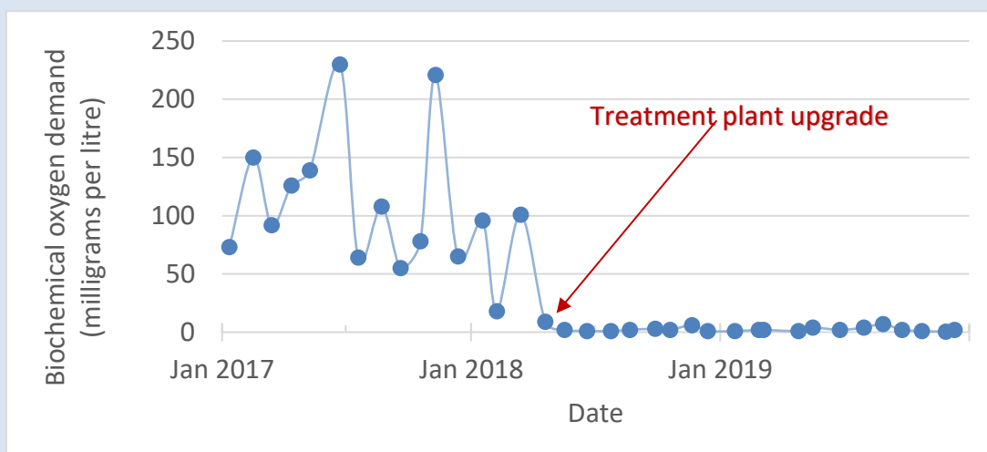
Figure 7: Effluent quality at Convoy.
