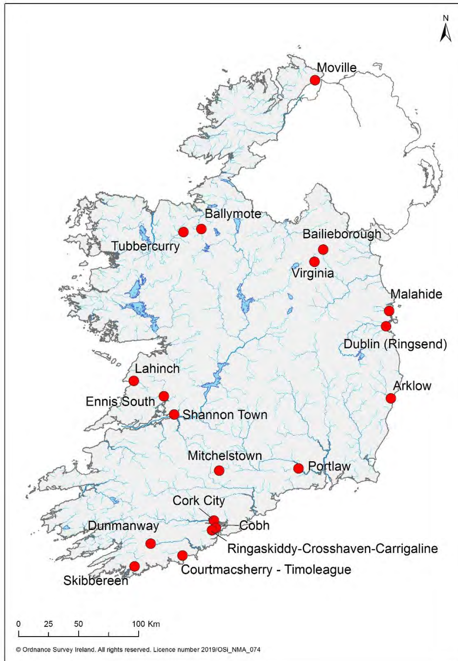
Figure 4: Large urban areas that failed to meet the European Union's treatment standards in 2019.
